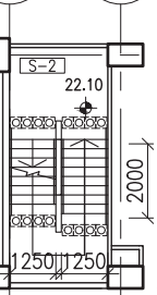
PART PLAN
